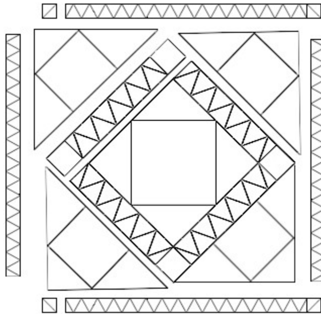
Assembly Diagram
